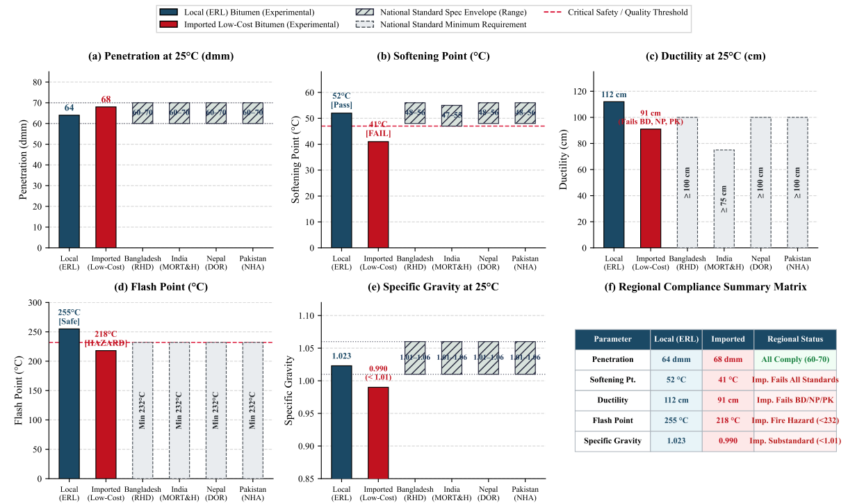
Figure 4.3: Comparative analysis of experimental physical properties of local (ERL) and imported low-cost bitumen against national highway specifications of South Asian countries (Bangladesh RHD, India MORT&H, Nepal DOR, and Pakistan NHA).
